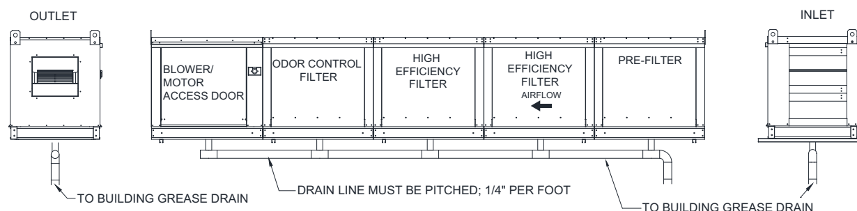
Figure 2 - Unit Drain Installation Details
