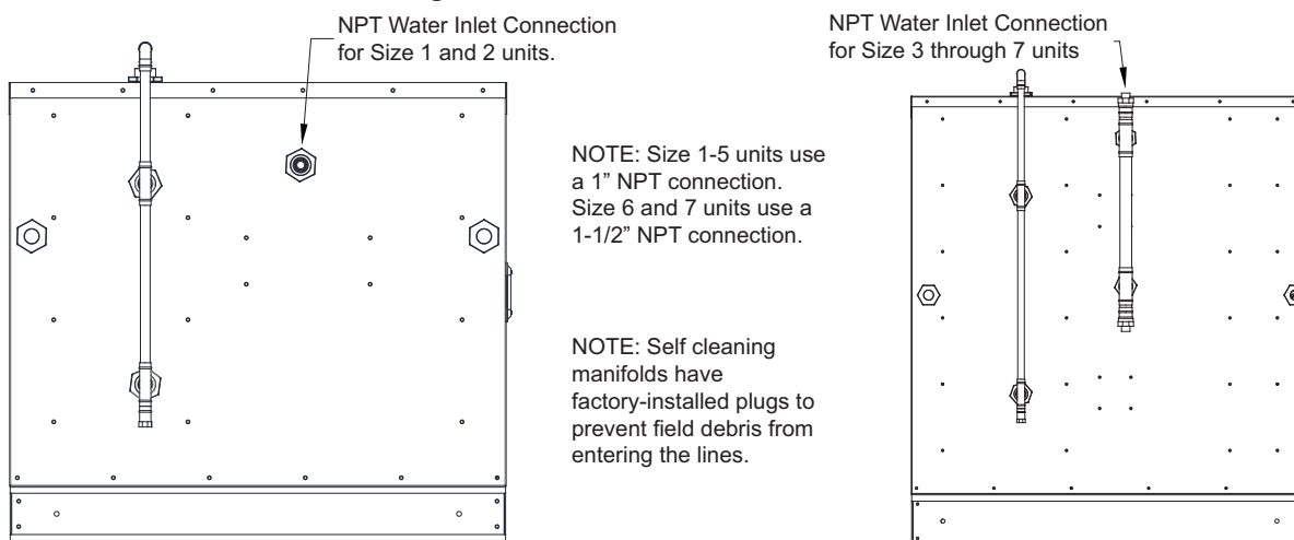
Figure 13 - Water Inlet Connection
