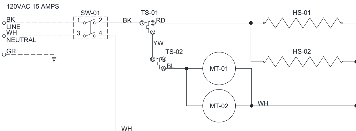
Figure 15 - Typical Wiring Schematic for Climate Controlled Utility Cabinet
