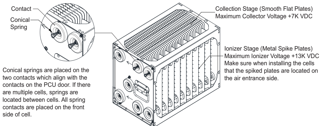
Figure 11 - ESP Cell
