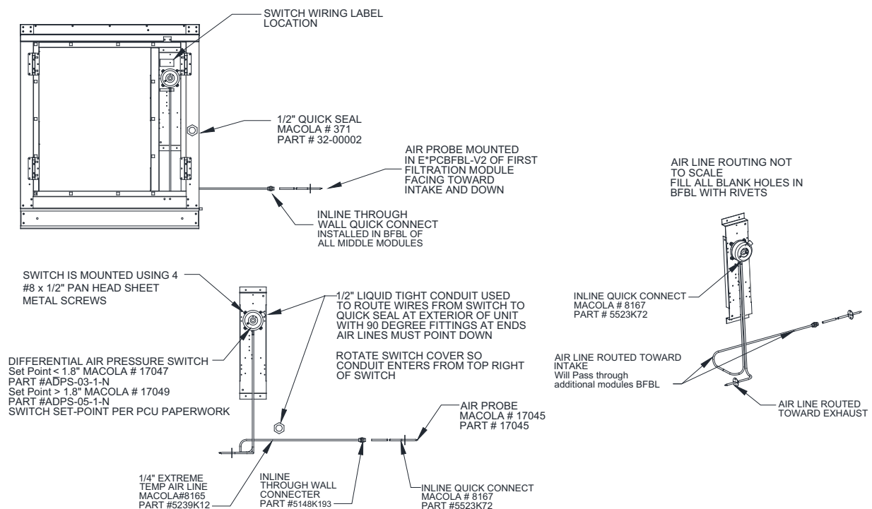
Figure 8 - Airflow Switch Installation
