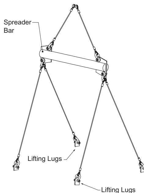
Figure 1 - Spreader Bar
