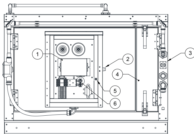
Figure 10 - ESP Module Components
