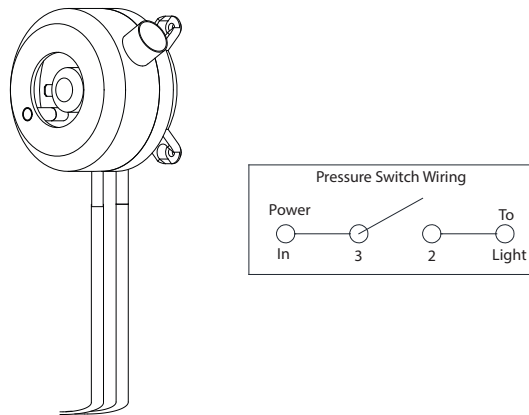
Figure 8 - Airflow Switch Installation
