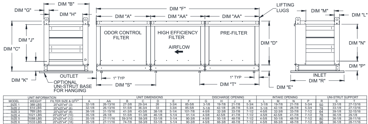
Figure 6 - Typical Indoor (Inline) Installation
