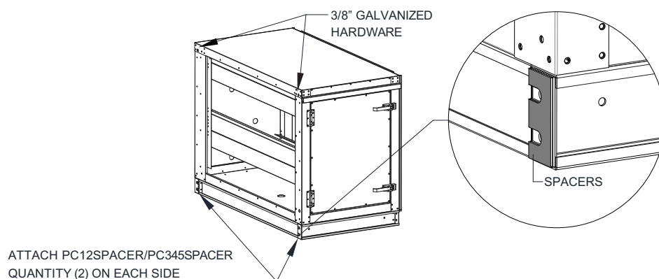
Figure 3 - Field Installation Details
